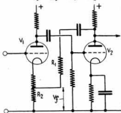
Fig. 5. Voltage feedback over two stages.
